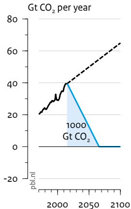
Linear reduction over about 50 years
