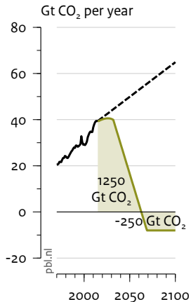
Negative emissions in the long term
